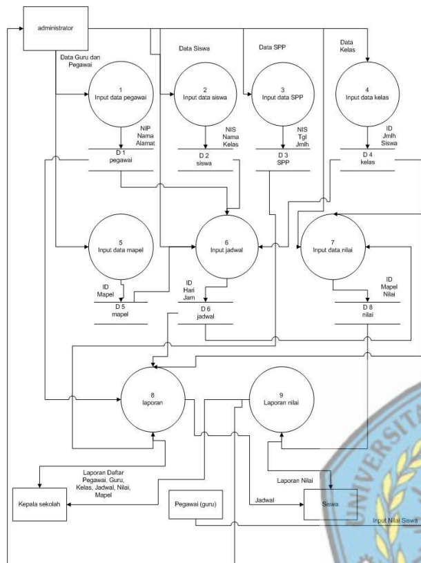
Gambar 3.3 DFD Level 1
