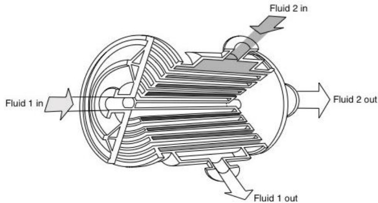
Gambar 2 7. Desain Heat Exchanger Plat Tipe Spiral
