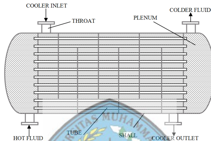
Gambar 2 1. Heat Exchanger Shell and Tube
