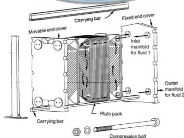
Gambar 2 3. Heat Exchanger Plat Tipe Gasket
