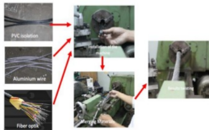
Fig. 2. Steps of twisting OPPC cable
