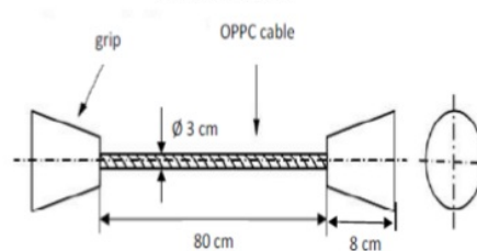
Fig. 4. The impact test specimens and tensile (SNI 07-0408, 1989)
