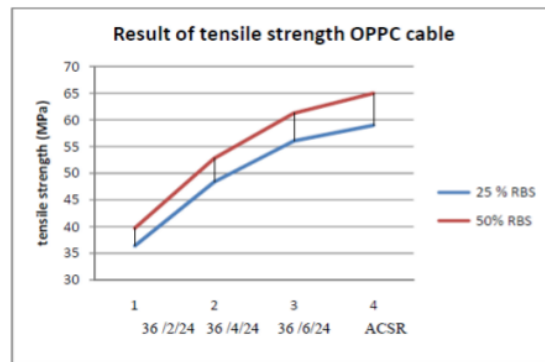
Fig. 6 Result of tensile strength OPPC cable
