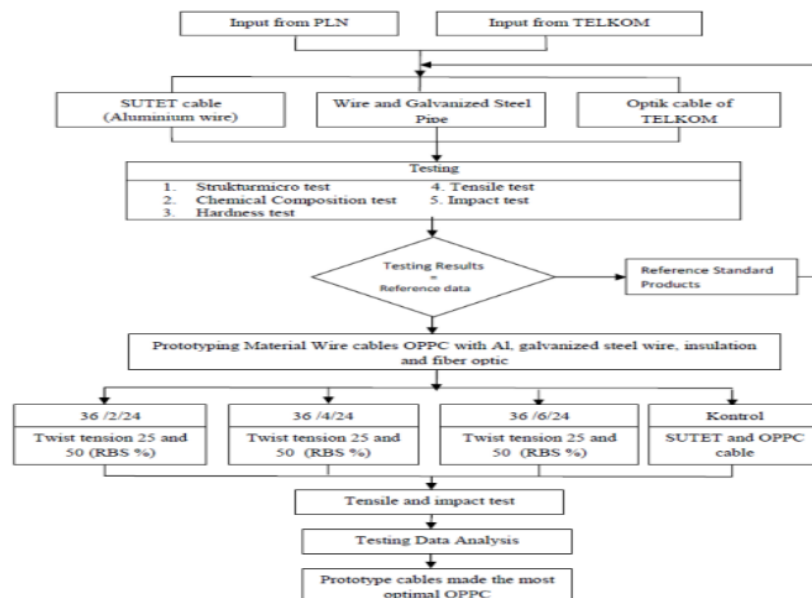
Fig 1. flow chart of manufacturing of OPPC cable
