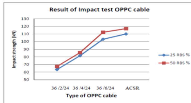
Fig. 5. Result of impact test OPPC cable
