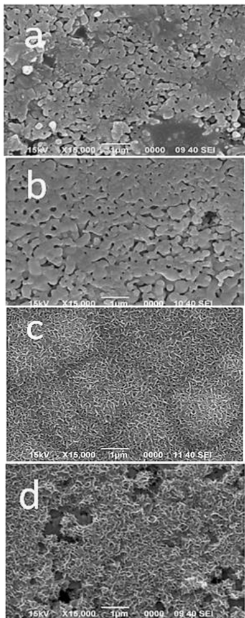
Figure 3. Surface morphology of sample after 336 hours immersed in SBF solution (a) 5wt% zeolite – HA, (b) 10 wt% zeolite – HA, (c) 25 wt% zeolite – HA, and (d) 50wt% zeolite – HA [40].
