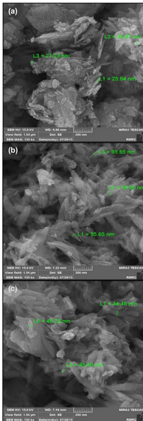
Figure 4. SEM morphology zeolit-HA nanocomposite with zeolite content of 2.5wt% (a), 5wt% (b), and 7.5wt% (c) [47].
