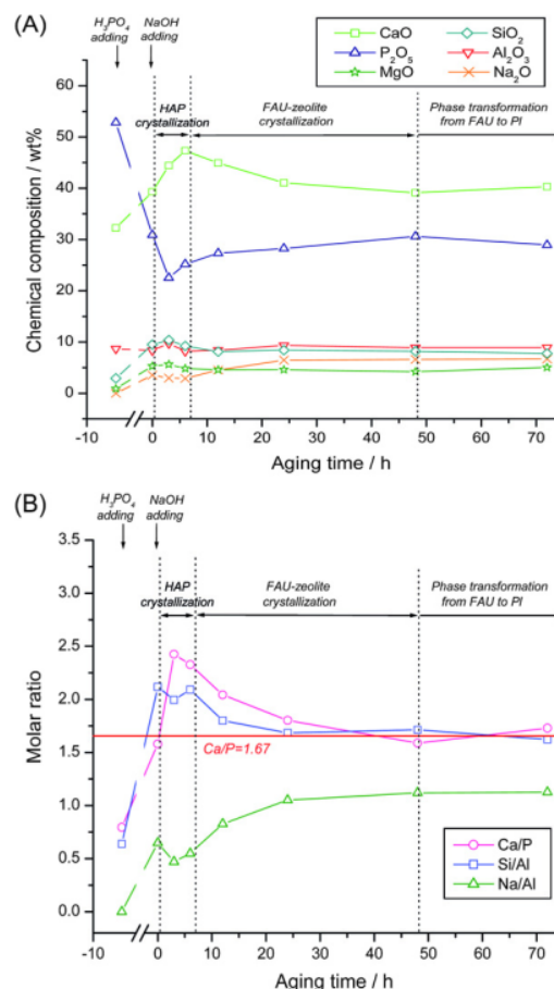
Figure 1. The relationship of alteration of chemical composition (A) and molar ratio of Ca/P, Si/Al and Na/Al against a change of aging time [44].
