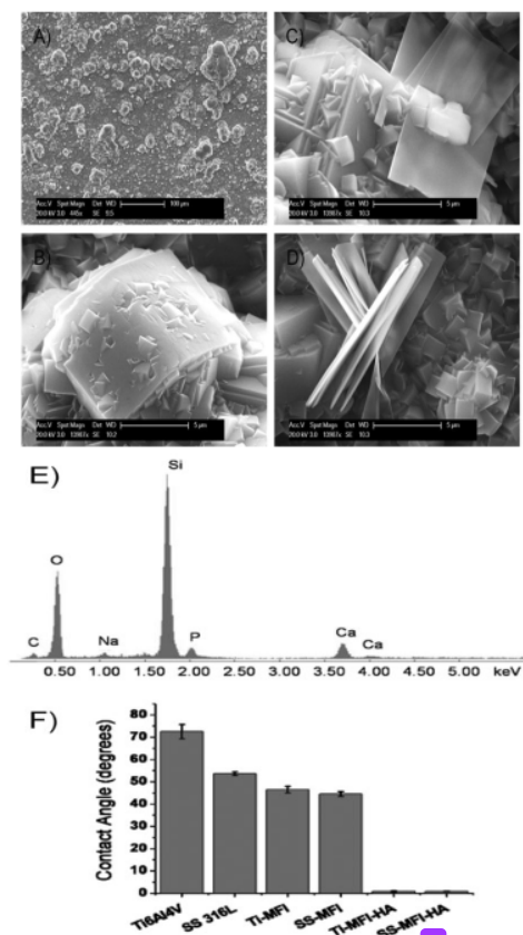
Figure 6. Surface morphology of (A) the coating of MFI-HA on Ti6Al4V substrate, (B, C) intergrowth on MFI-HA surface for 4 hours MFI synthesized, (D) MFI-HA surface intergrowth after 4 hours MFI synthesized, (E) HA crystalline structure observed after 4 hours MFI synthesized. (F) The contact angle of MFI-HA coating, MFI coated, and uncoated Ti6Al4V substrates [73].
