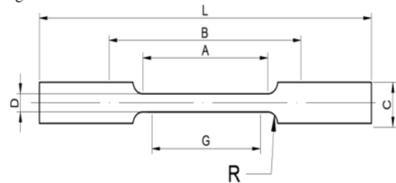
Figure 1: Tensile Strength Testing Specimen
