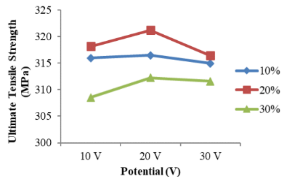
Figure 3: The relationship between ultimate tensile strength for anodizing results with different concentrations of electrolyte solutions
