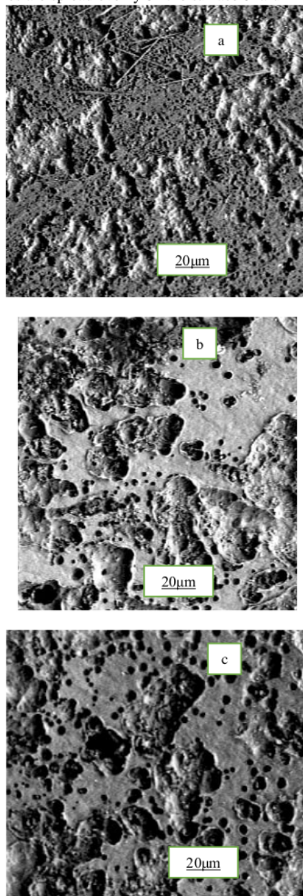
Figure 5: Surface morphology of AA 6061 T6 after anodizing at 20 V potential and different concentrations of sulfuric acid (a) 10% (b) 20% (c) 30%
