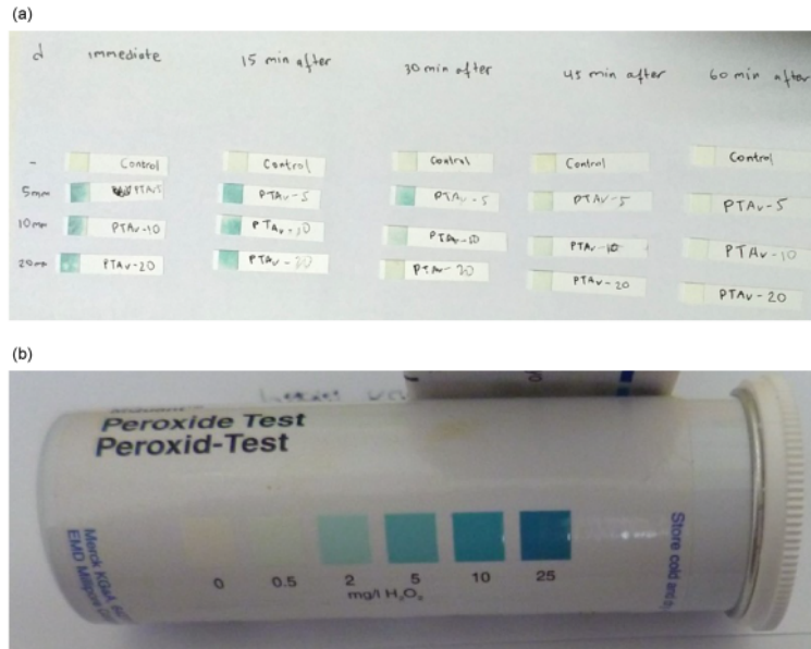
FIG. 5: (a) representative semiquantitative conditions of H_2O_2 on surface of aloe vera slice for 60 min following plasma jet treatment. H_2O_2 detected immediately and 15 min post-treatment in PTA-5, PTA-10, and PTA-20 but not detected 45 min and 60 min post-treatment. At 30-min post-treatment, H_2O_2 detected in PTA-5 but not in PTA-20. PTA-5: plasma jet-treated aloe vera slice at 5-mm distance; PTA-10: plasma jet-treated aloe vera slice at 5-mm distance; PTA-20: plasma jet-treated aloe vera slice at 20-mm distance. (b) H_2O_2 indicator.
