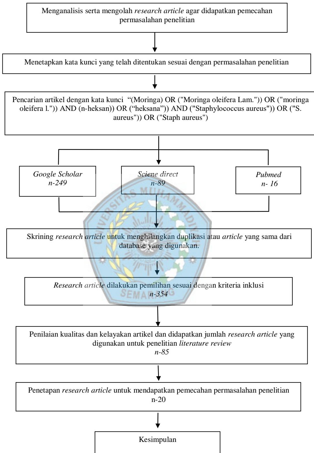
Gambar 2.1. Prosedur Penelitian
