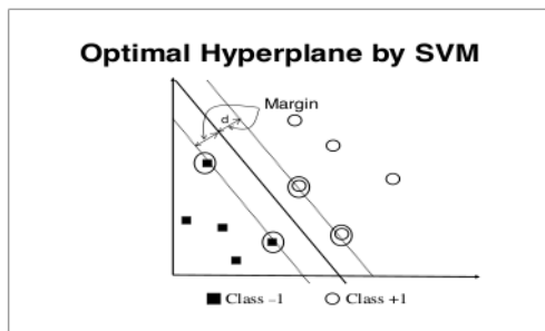
Figure 1. Optimal hyperplane by SVM
