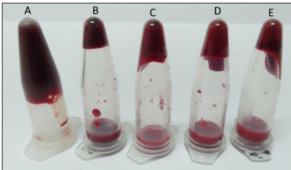
Figure 3. Blood clot-lysis test results using bacterial crude enzyme; A - blood clot without addition of enzymes (control); B - blood clot with addition of 100 \mu\text{L} nattokinase; C - blood clot with addition of 100 \mu\text{L} crude 100% enzyme; D - blood clot with addition of 200 \mu\text{L} crude 100% enzyme; E - blood clot with addition of 300 \mu\text{L} 100% crude enzyme.
