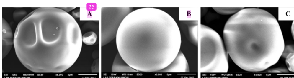
Fig (1). SEM micrograph of microcapsules with (A) MDE-AG; (B) MDE-AG-βCD; and (C) MDE-βCD
