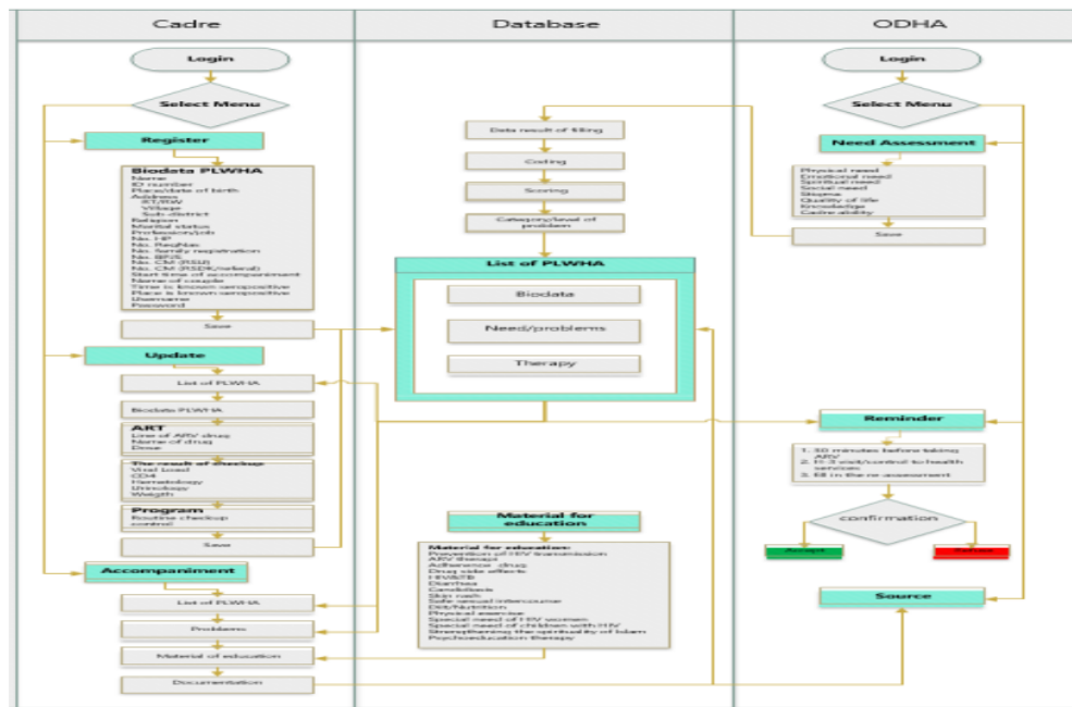
Fig.2: The SEHAT-Kader data management program
