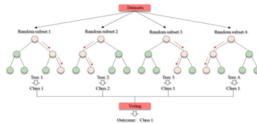
Fig. 2. Illustration of Random Forest Algorithm [39]
